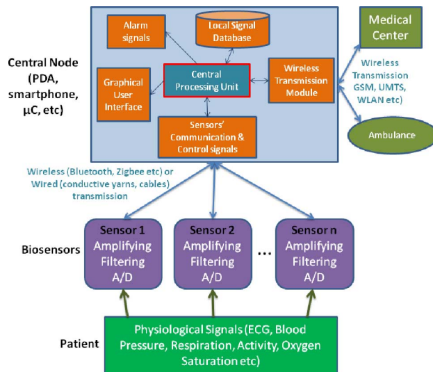
Fig. 1. Architecture of a wearable health-monitoring system.
